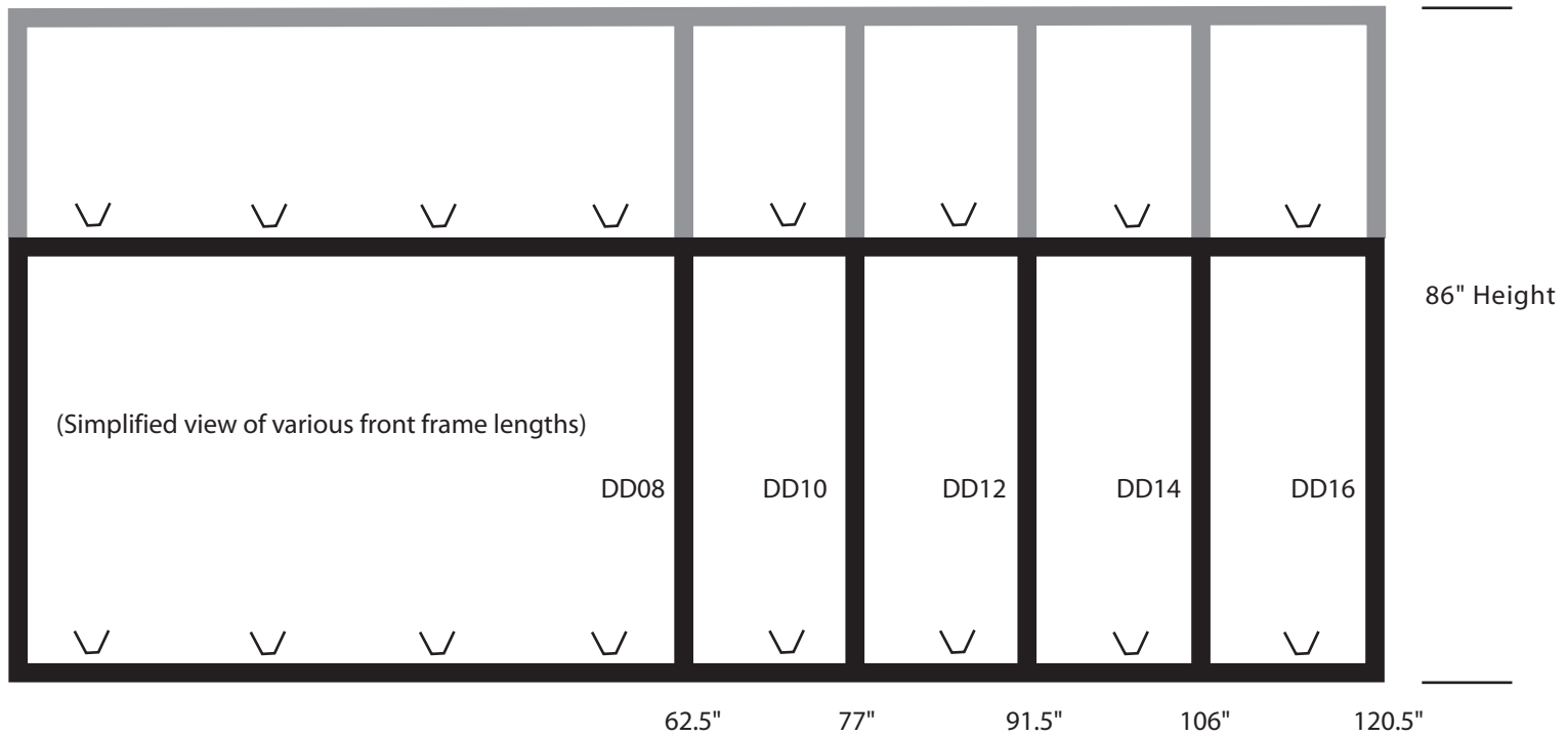
Front View
